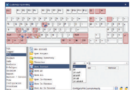
Custom Keybinding
